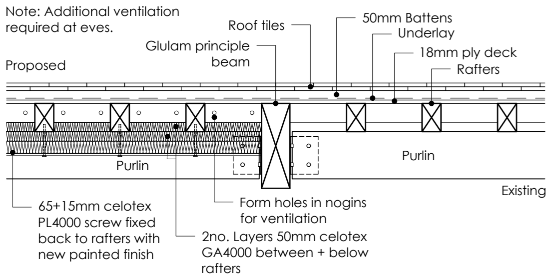
Detail 01 - Proposed ceiling insulation (Note: All sizes approximate: Not measured)
